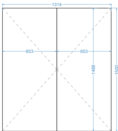
Elevations exterieures
